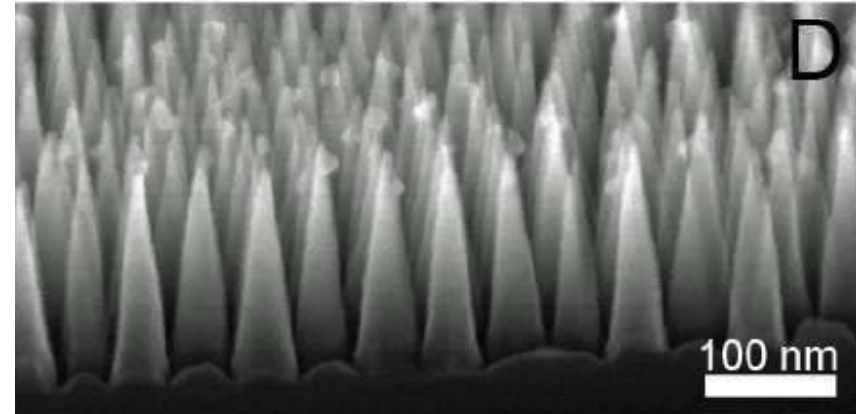
Superhydrophobic surfaces
